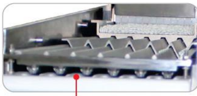
PMC 40 Dust Extractor
